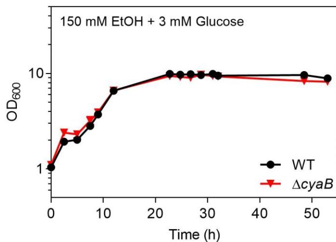
FIGURE S2. Growth of C. glutamicum WT and the \Delta cyaB mutant in CGXII minimal medium with 150 mM ethanol and 3 mM glucose. Cultivation was performed in baffled shake flasks that were incubated at 30 °C and 120 rpm at 85% humidity. Mean values and standard deviations of three biological replicates are shown.
